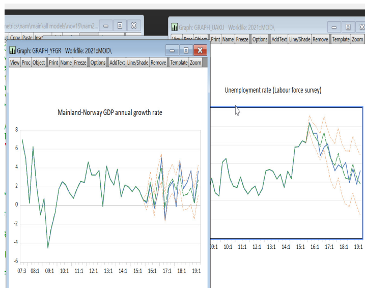
Figure 4.4: Screen capture of two graphs with within sample simulation results, produced by running a NAM-prg file with %FSTART set to 2016q1 and %FSTOP to 2019q3.
